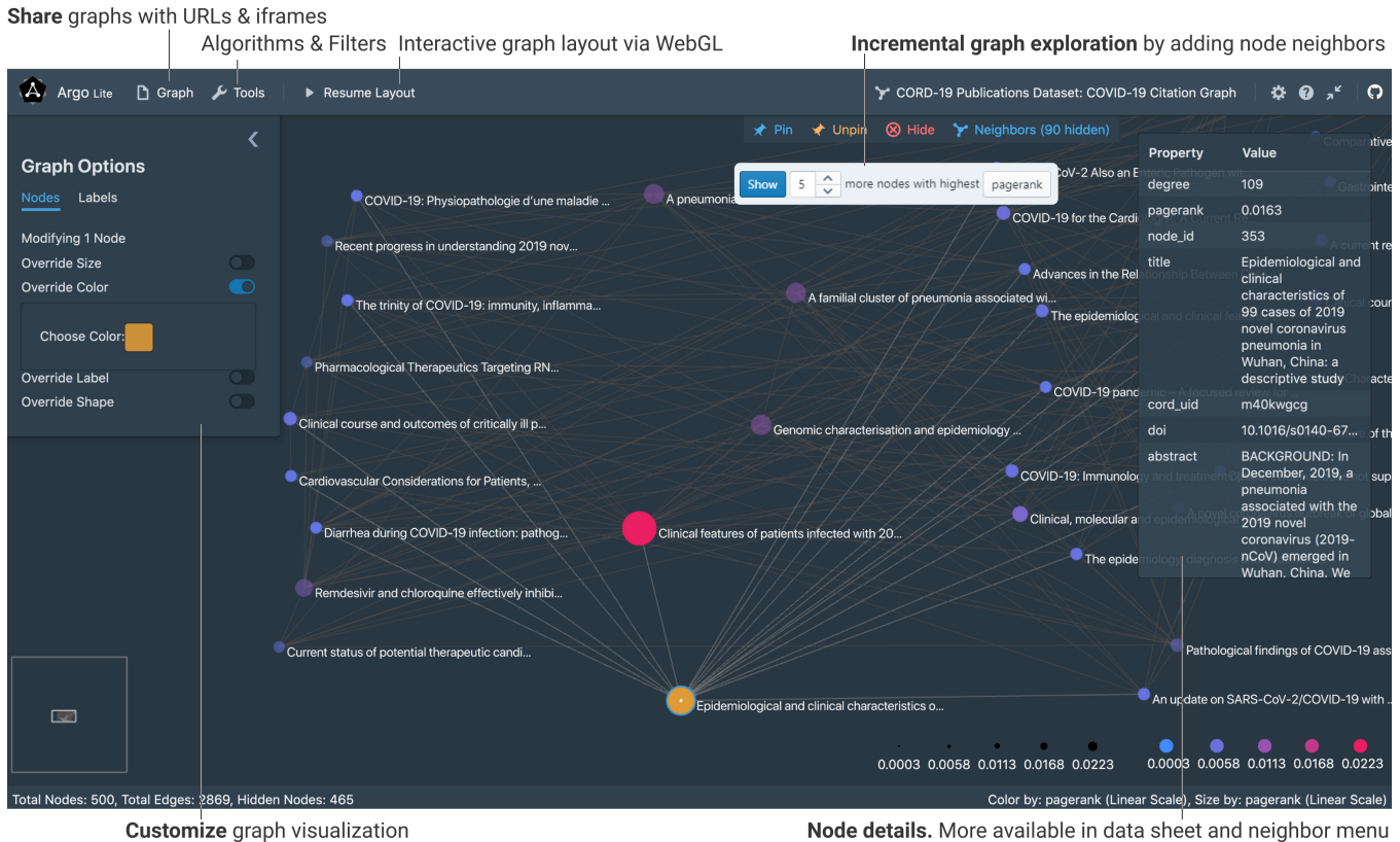
Figure 1: ARGO LITE visualizing a citation network of recent COVID-19 publications [12]. ARGO LITE users can explore graphs incrementally by adding more related papers (e.g., highly cited papers cited by or citing a paper of interest) to the visualization [3]. Using WebGL for high-performance cross-platform graph rendering [4], ARGO LITE runs in all modern web browsers without requiring any installation.
