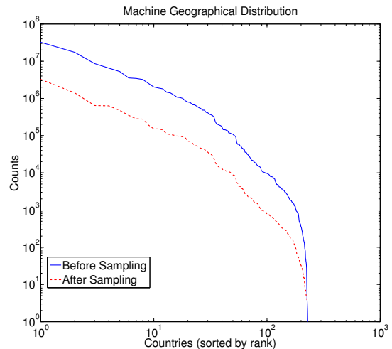
Fig. 4. Distribution of machines per country, in log-log scale. We have anonymized the countries, for privacy purposes, with the total number of countries in WINE being 229. The distribution follows the GEOSPLIT model, as we describe it in Section III of the text and the appendix. We observe that both the sampled and the original data follow the same distribution, with obvious displacements due to sampling.
