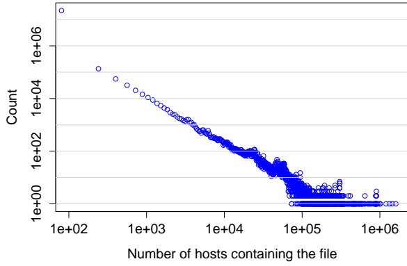
Fig. 1. Distribution of file popularity among machines. We observe that the popularity of a file, which also reflects its volume on the database, follows a power law.
