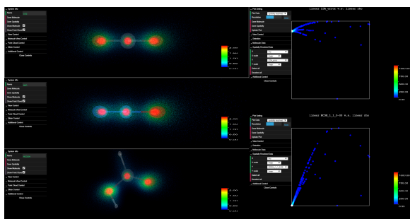
Figure 2: ElectroLens simultaneous viewing atomistic (spheres) and electronic environments (point cloud) for multiple systems. The chemical systems shown are carbon dioxide ( \text{CO}_2 ) (top), nitrous oxide ( \text{N}_2\text{O} ) (middle), and formic acid ( \text{HCOOH} ) (bottom). The 2D plots show the error of an ML model vs. electron density (top) and the first derivative of the electron density vs. electron density (bottom). Features in the 2D plots correspond to all 3 systems.
