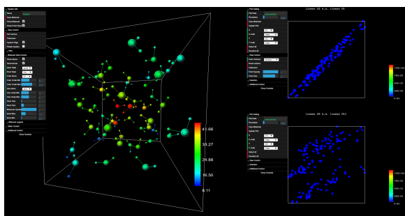
Figure 4: ElectroLens visualizing a cluster of water ( \text{H}_2\text{O} ) molecules. For the 3D view, the size codes atom type (large = oxygen, small = hydrogen), and the color codes the values of a symmetry function fingerprint [8]. The lines between atoms label the bonds. Both 2D plots are plotting two symmetry function features, and users can select parts on the 2D plots to view the corresponding atoms in the 3D view.
