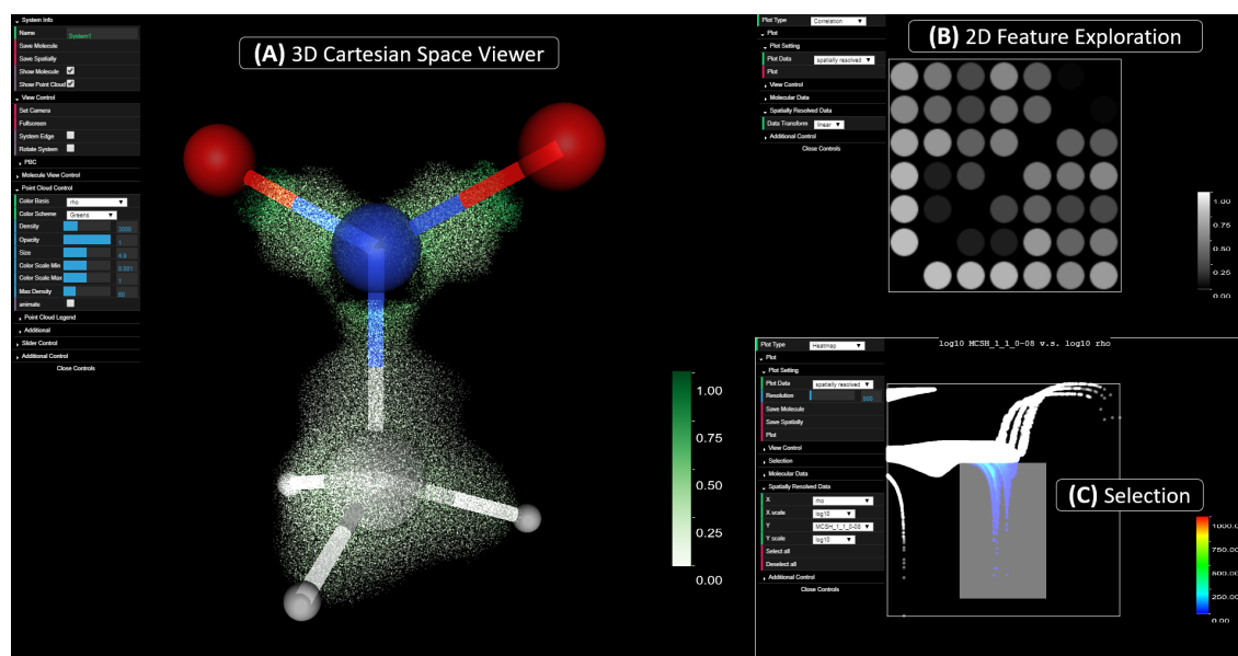
Figure 1: The ElectroLens user interface (UI) visualizing the electron cloud of \text{CH}_3\text{NO}_2 molecule. The UI has two main parts: 3D viewer(s) on the left, and 2D plots on the right with option boxes in each view for customization. (A) The 3D viewer for Cartesian space. ElectroLens uses a “point cloud” to mimic the electron cloud, where the density of points corresponds to the density of electron cloud, and the color corresponds to energy density in this case. ElectroLens utilizes the ball-and-stick model to visualize atoms, where different atom types are denoted by white (hydrogen), grey (carbon), blue (nitrogen), and red (oxygen) spheres. (B) 2D plots for exploring and plotting additional features. The upper plot is the correlation plot used to identify the potentially interesting combinations of features. The plot below is a scatter plot of two features (in log-scale), where the color codes the number of data points represented. (C) Selecting parts on the scatter plot causes the corresponding points in 3D viewer and other scatter plots to be highlighted. This case illustrates the connection between the features (right) and the chemical concept of a C-N bond (left).
